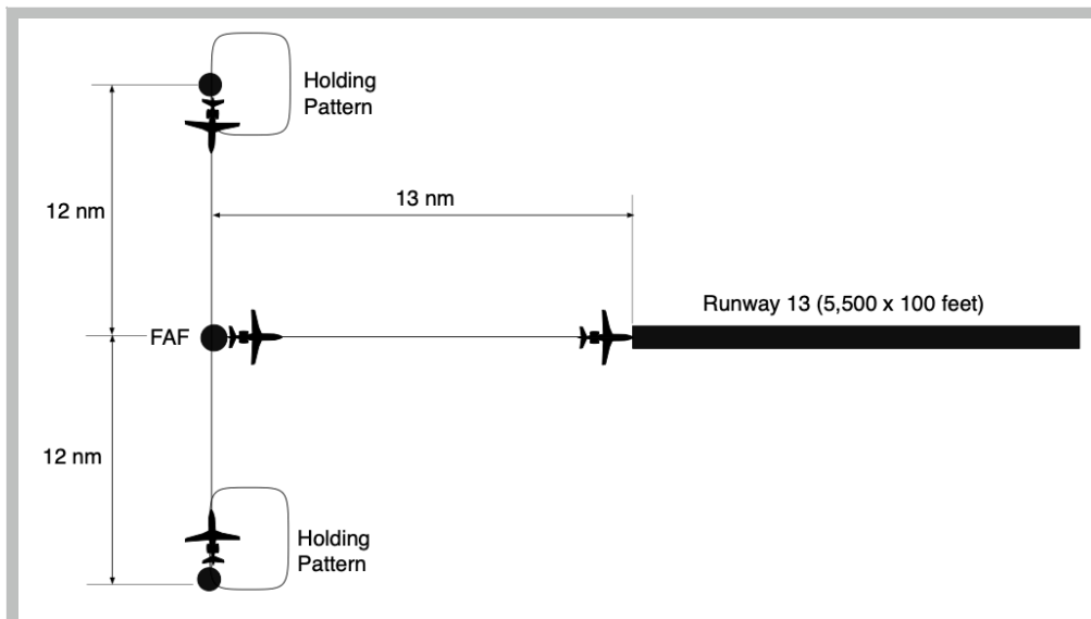
Figure 1. Runway and Airspace Configuration for Problem 1.
