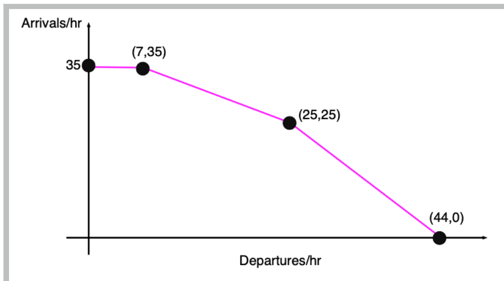
Figure 2. Arrival-Departure Diagram for Problem 2.
