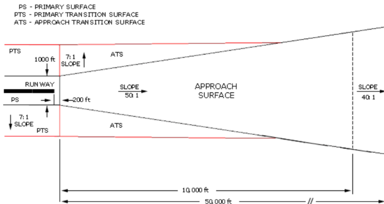
PIR PRECISION INSTRUMENT APPROACH
