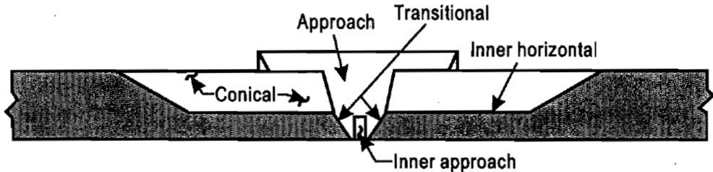
Section B-B
