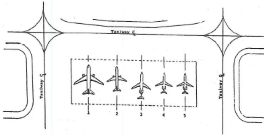
Figure 3-2. Example of a common deicing pad layout
