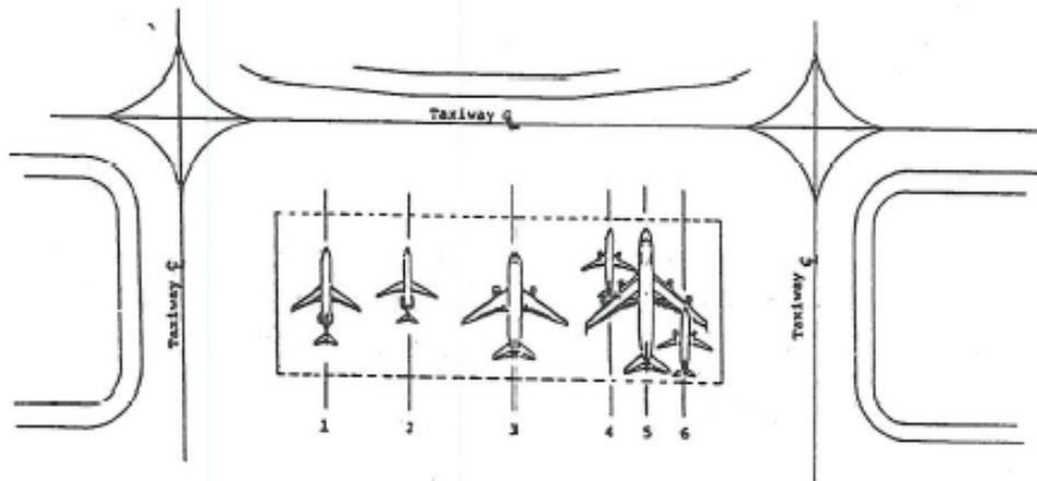
Figure 3-3. Example of a composite deicing pad layout
