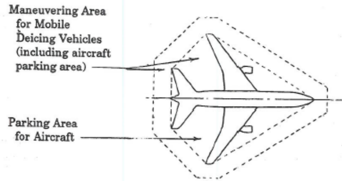
Figure 1-1. Aircraft deicing pad with vehicle maneuvering area
