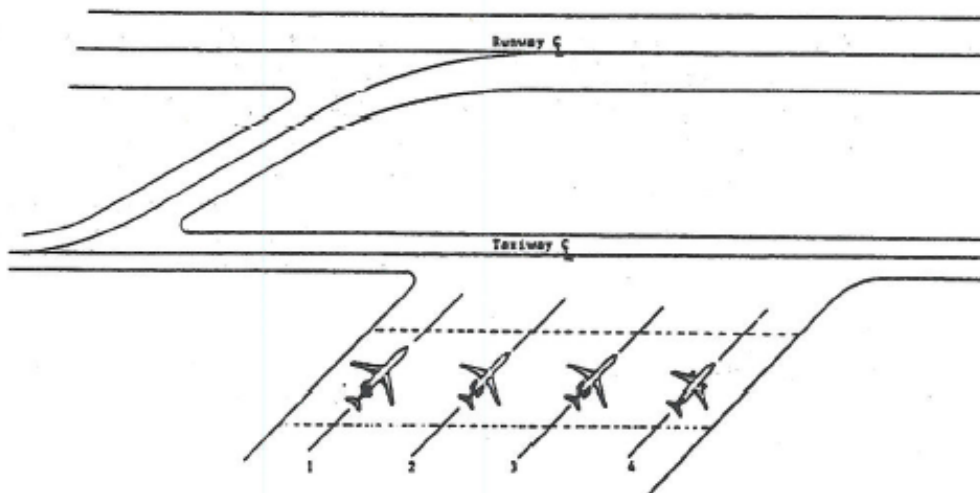
Figure 3-4. Deicing pad centerlines oriented 45 degrees to the connecting taxiway
