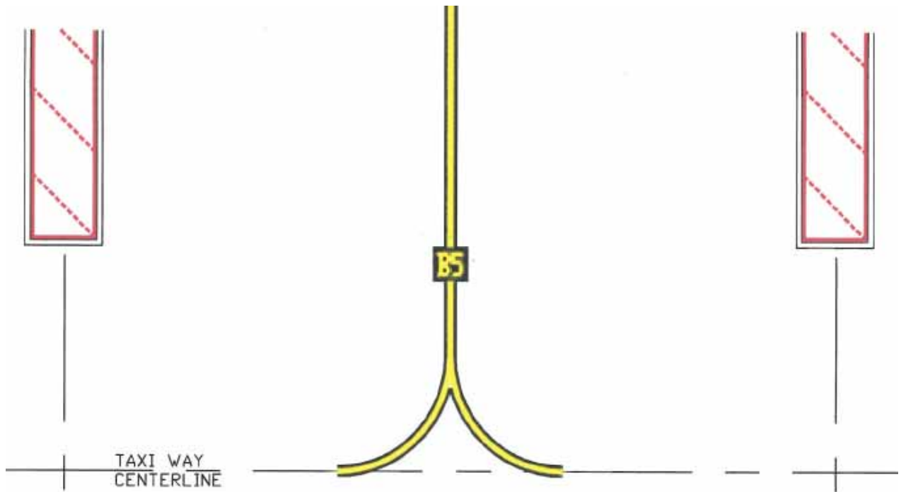
Figure 3-1(b). Deicing pad identification (“B5”) surface marking at entrance point
