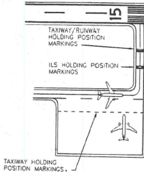
Figure 3-1(a). Facility taxiway/taxiway holding position marking
