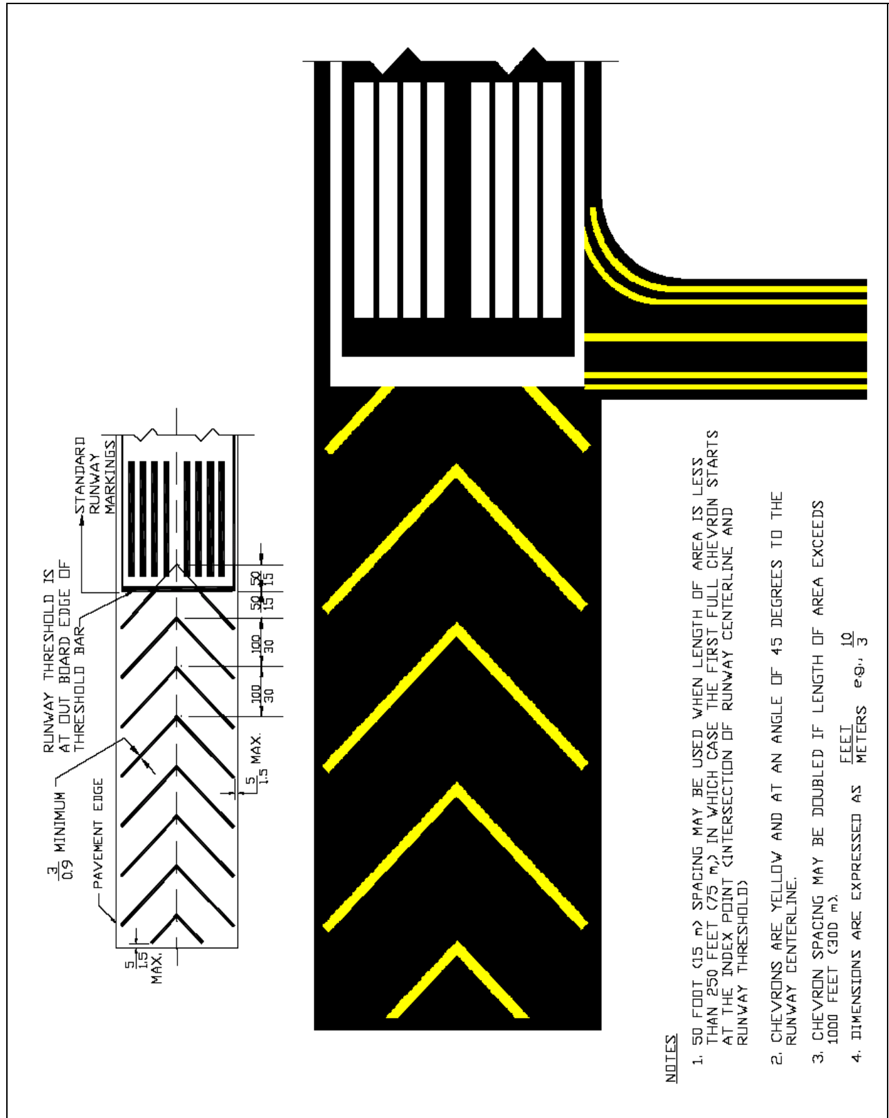
Figure 7. Markings for Blast Pads and Stopways
