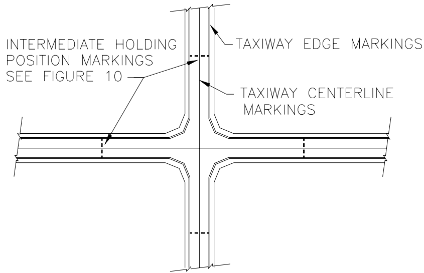
A. EXAMPLE OF TAXIWAY CENTERLINE MARKING AT INTERSECTION HAVING LESS THAN STANDARD FILLETS AND REQUIRING JUDGMENTAL OVERSTEERING
